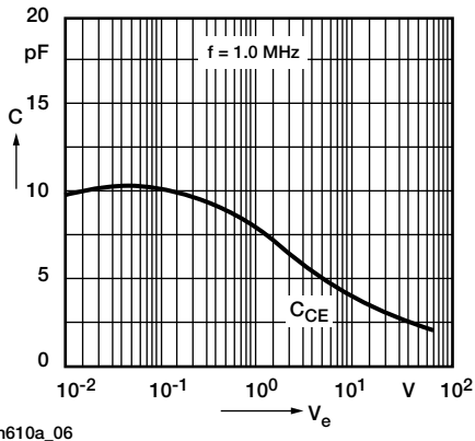
isfh610a_06 Fig. 6 - Transistor Capacitance (Typ.) vs. Collector Emitter Voltage
