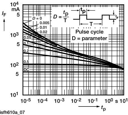
isfh610a_07 Fig. 7 - Permissible Pulse Handling Capability Forward Current vs. Pulse Width
